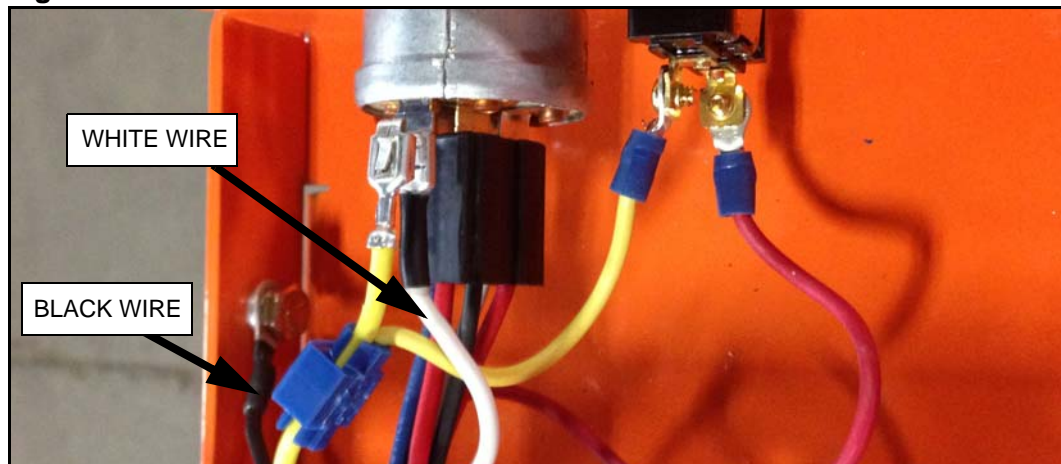
Figure 1.1 Control Box Connections
